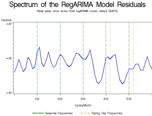
Figure 3: Spectrum plot of the final 8 years of the regARIMA residuals with trading day regressors included in the model of Retail Shoe Store Sales.
